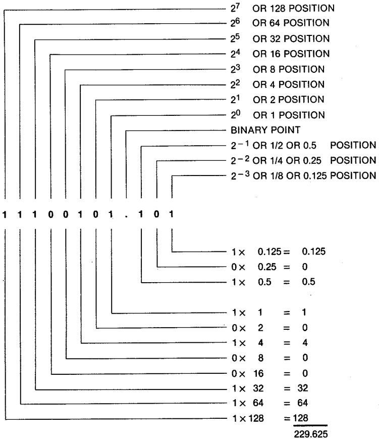
Fig. 2-5. Extending binary notation to include fractions.
